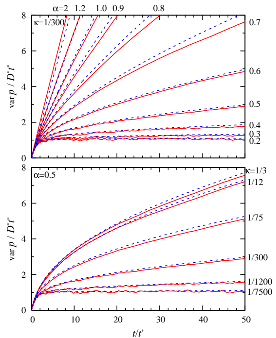
FIG. 1: (color online). Time dependence of the momentum spreading \text{var } p(t) for kicked rotators which are subjected to Lévy noise generated by a Yule-Simon distribution. The results of numerical simulations (solid curves) are compared to the theoretical predictions from Eq. (6) (dashed curves). In the upper panel, the exponent \alpha varies while the noise strength \kappa = 1/300 is fixed. The bottom panel shows results for fixed \alpha = 0.5 and varying noise strength \kappa .
